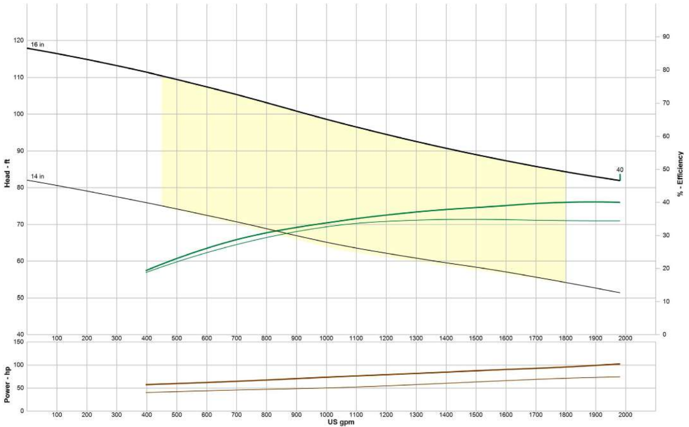
EDDY Pump - 6-Inch DEP 6000 Diver Operated Dredge - Pump Curve
