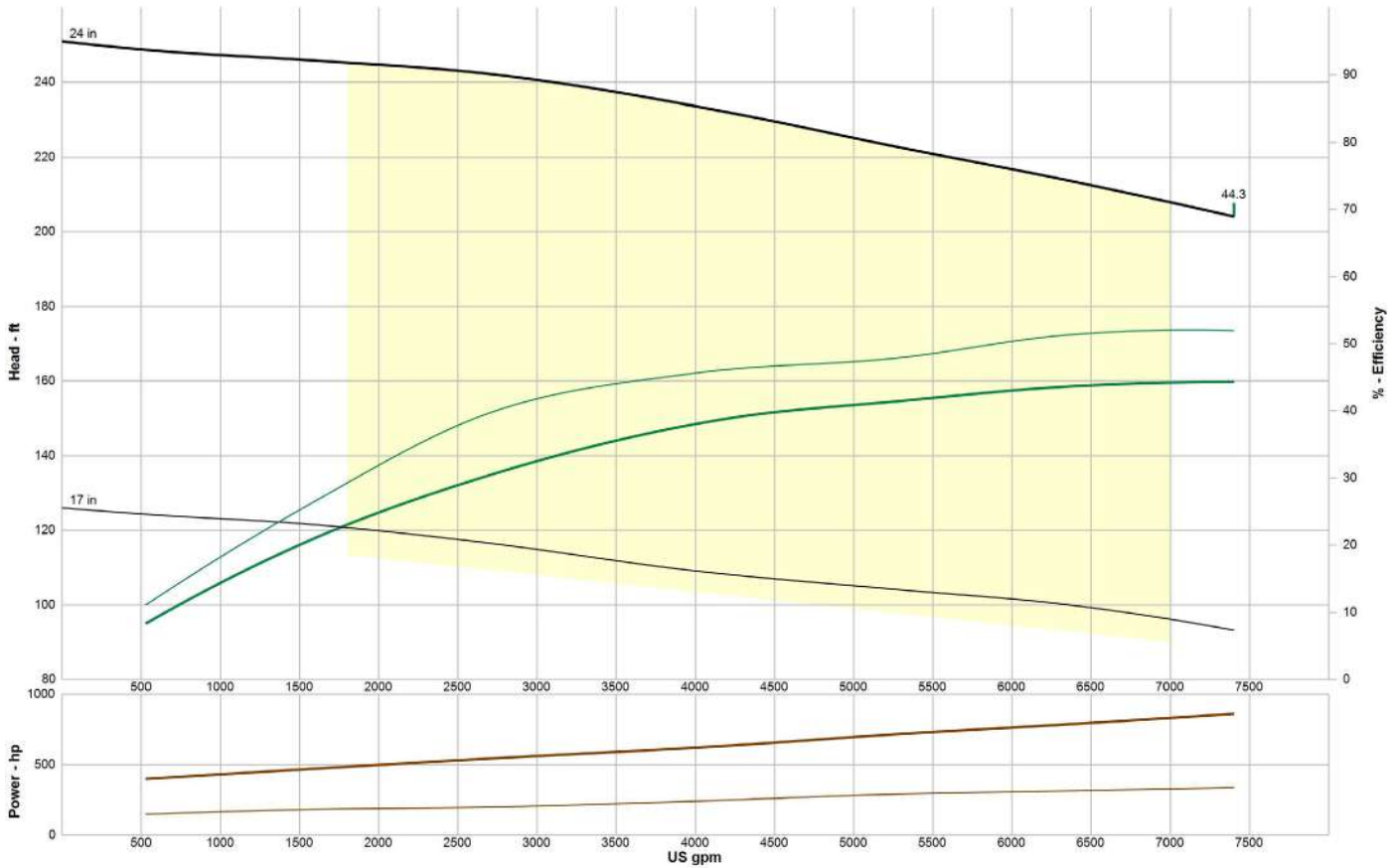
EDDY Pump - 12 Inch EXH 12000 Hydraulic Excavator Attachment - Pump Curve
