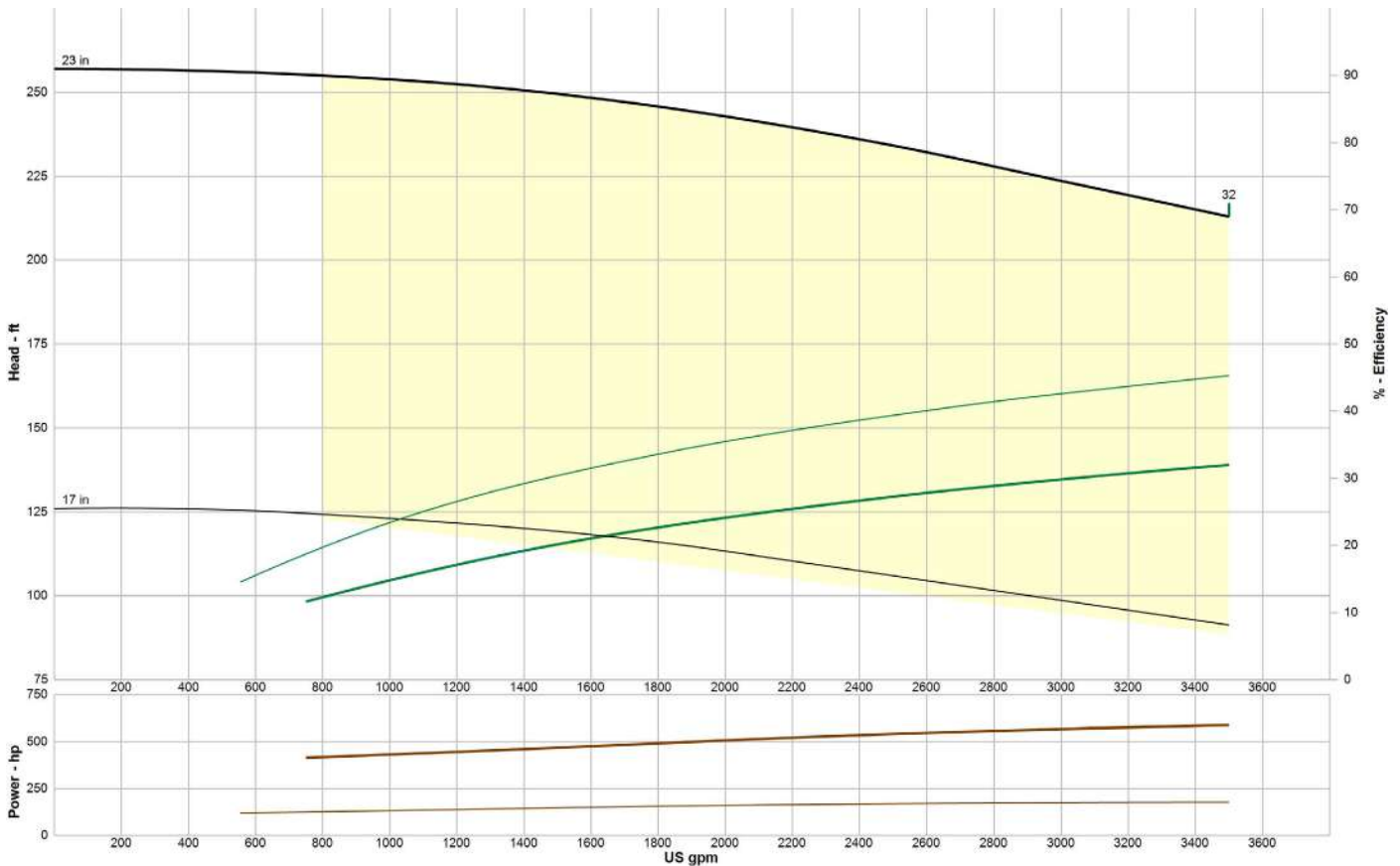
EDDY Pump - 8 Inch Subdredge - Pump Curve
