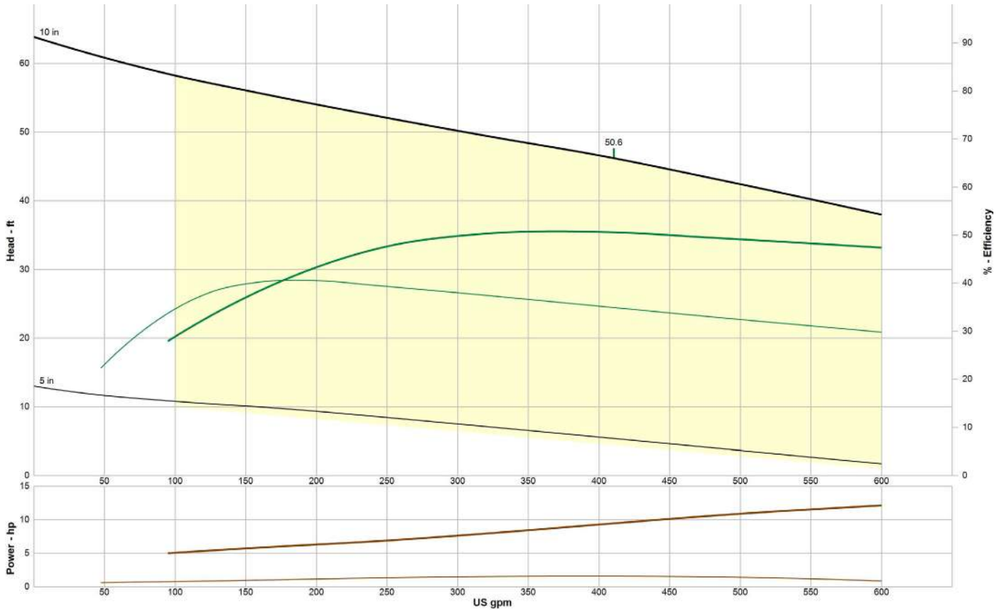
EDDY Pump - 3 Inch C 3400 Commercial Slurry Pump - Pump Curve
