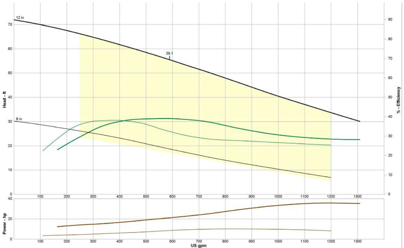
EDDY Pump - 4 Inch C 4600 Commercial Slurry Pump - Pump Curve
