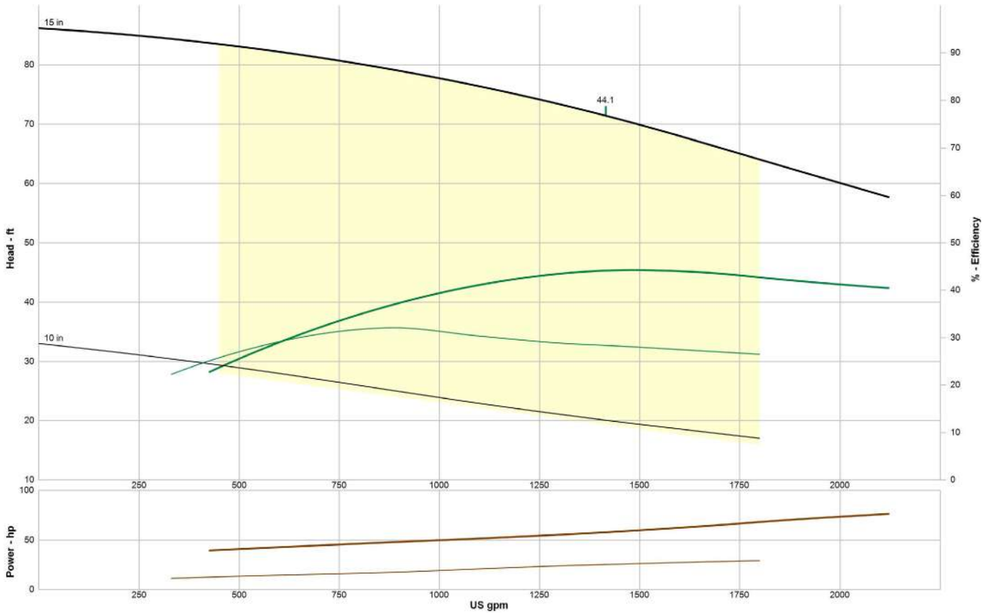
EDDY Pump - 6 Inch C 6800 Commercial Slurry Pump - Pump Curve
