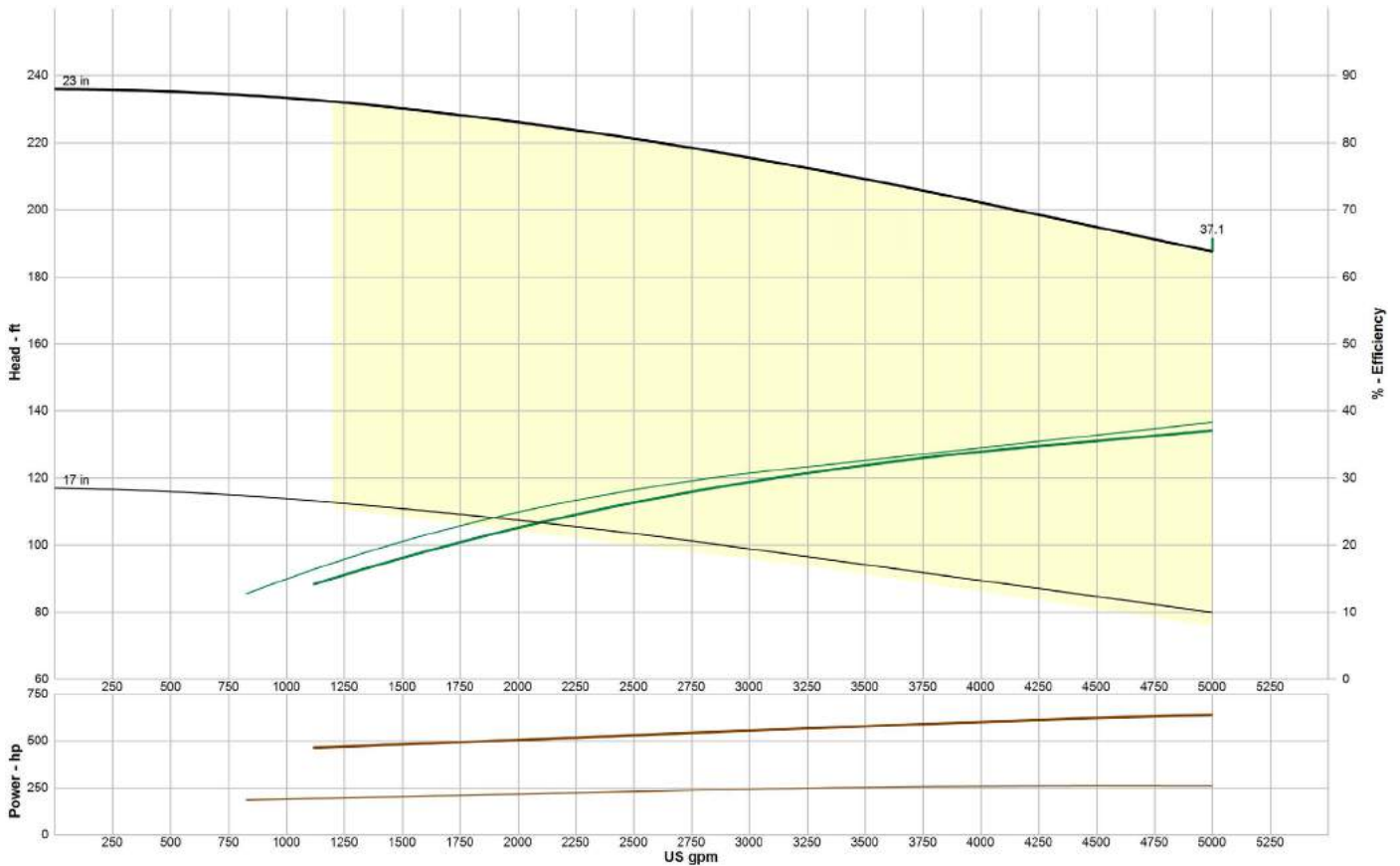
EDDY Pump - 10 Inch JPH 10000 Cable Deployed Pump - Pump Curve
