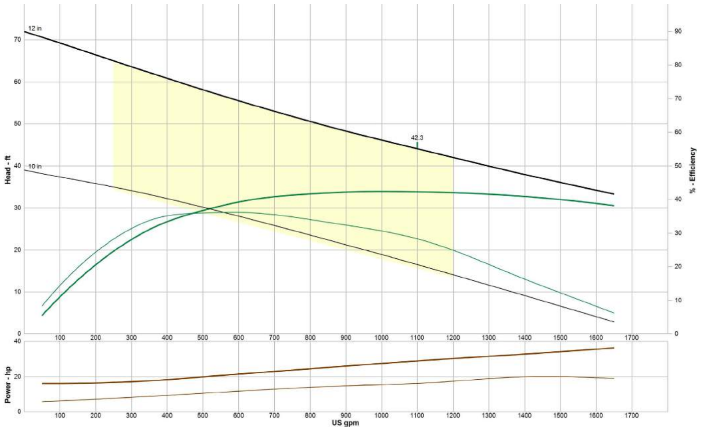
EDDY Pump - 4 Inch JPH 4000 Cable Deployed Pump - Pump Curve
